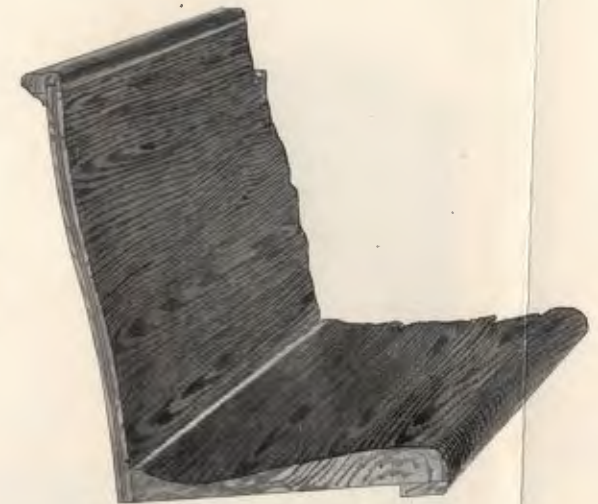
Pew Body No. 3. Three-ply resawed back. Made either single or compound curved; for straight pews only.
